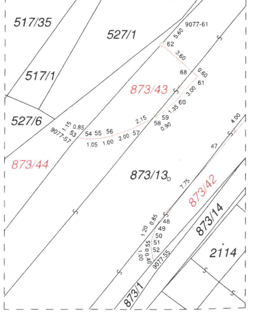
Detail A
